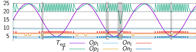
Figure 6: A trace of simulation: T and T_{ext} represent the inside and outside temperatures, Op_i corresponds to heater i being operational and On_i corresponds to heater i being switched on. Gray areas highlight failure of at least one heater when T_{ext} < T_{min} .
