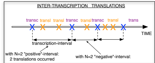
Figure 3: Inter-transcription translations
