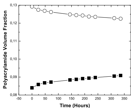
Figure 6: Time evolution of polymer volume fraction in both tubes for \bar{\varphi}_p = 0.1072 . \blacksquare , top tube ; \circ , bottom tube ; solid lines represent fits by ?? ( T = 298 K, polymer from batch #1).
