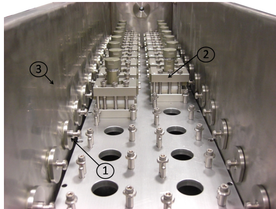
Figure 2: Photograph of the chamber containing the sets of tubes. (1) Screws used to switch between "faced" and "separated" positions, (2) Sets of sliding tubes, (3) Insulated walls.
