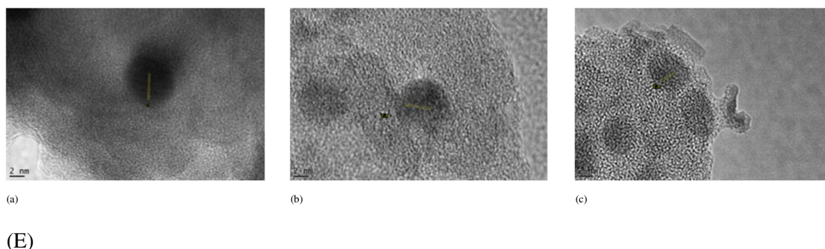
Figure 6. (A) TGA plots of the catalysts after activity tests at 750°C, (B) Carbon deposition calculated from TGA on different catalysts, (C) TEM micrographs, (D) Ni particle size distribution after CRM test at 750°C and (E) HRTEM micrographs (a) Ni/SBA-16-WI, (b) Ni/SBA-16-CA, and (c) Ni/SBA-16-AE.
