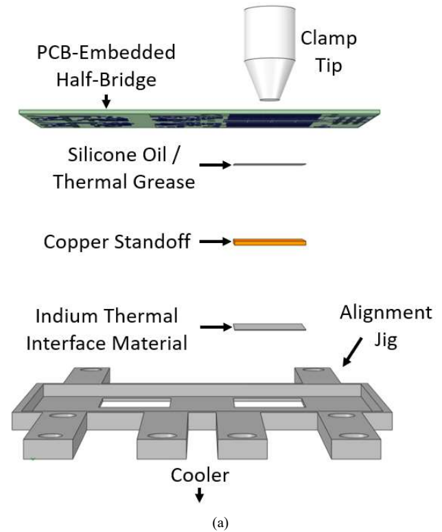
Fig. 3. (a) An exploded side view of the heating characterization test setup and (b) an example of the PCB-embedded half-bridge module mounted to the liquid cooled test fixture for a heating characterization test.
