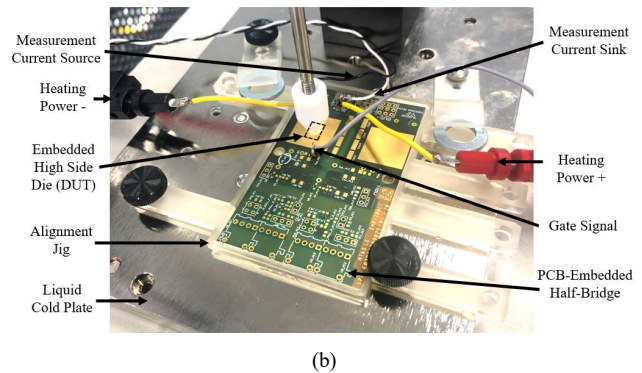
Fig. 3. (a) An exploded side view of the heating characterization test setup and (b) an example of the PCB-embedded half-bridge module mounted to the liquid cooled test fixture for a heating characterization test.
