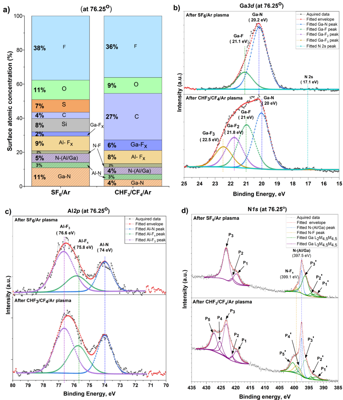
Fig. 6. (a) Surface atomic concentration and (b) Ga3d, (c) Al2p, and (d) N1s core levels spectra of the AlGa N surface after SiN etching by high-energy SF 6 /Ar and high-energy CHF 3 /CF 4 /Ar plasma processes measured by AR-XPS at a grazing angle of 76.25°.
