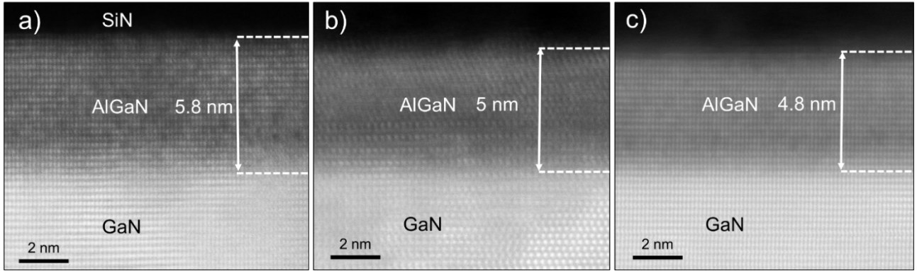
Fig. 15. Cross-section TEM image of the AlGaIn/GaN layers for (a) Before SiN etching (b) sample after low-energy SF 6 /Ar plasma etching followed by KOH treatment and (c) sample after low-energy CHF 3 /CF 4 /Ar plasma etching followed by KOH treatment.
