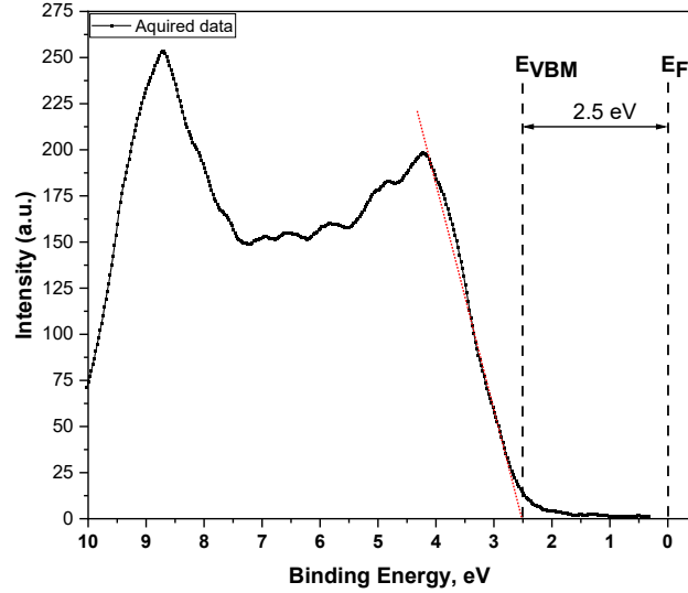
Fig. 5. Valence-band spectrum for the reference AlGaIn sample.
