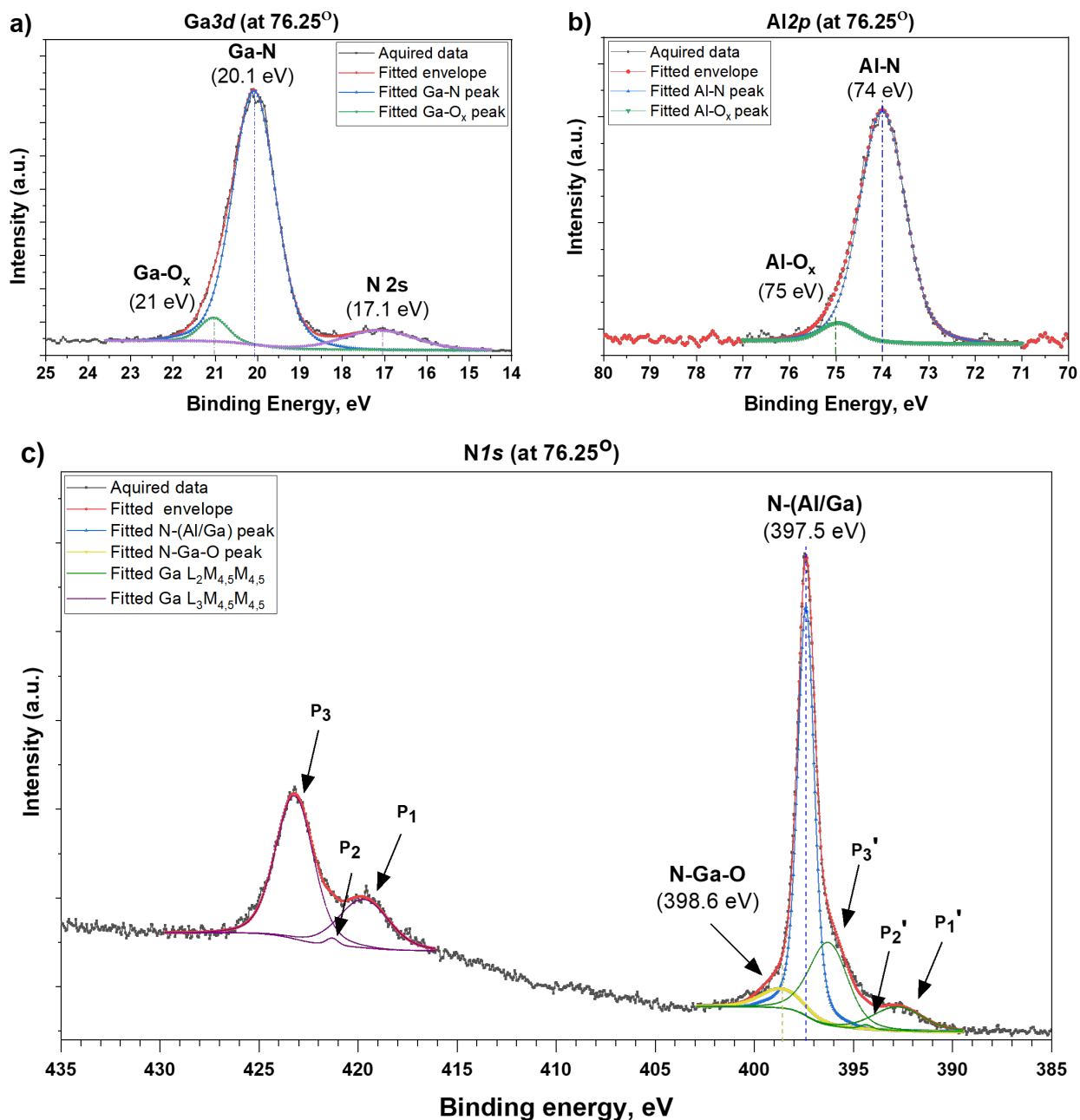
Fig. 4. (a) Ga3d , (b) Al2p , and (c) N1s core levels deconvolution of AR-XPS spectra of the reference AlGa 3 N sample measured at 76.25°.
