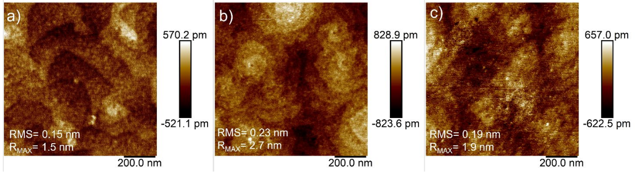
Fig. 16. AFM measurements of the AlGaIn surface for (a) reference sample (after BOE) (b) sample after low-energy SF 6 /Ar plasma etching followed by KOH treatment, and (c) sample after low-energy CHF 3 /CF 4 /Ar plasma etching followed by KOH treatment.
