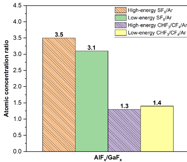
Fig. 9. The Al-F x /Ga-F x ratio of the AlGa n N surface after low-energy SF 6 /Ar and low-energy CHF 3 /CF 4 /Ar plasma etching extracted from the AR-XPS spectra measurements at surface grazing angle 76.25°.
