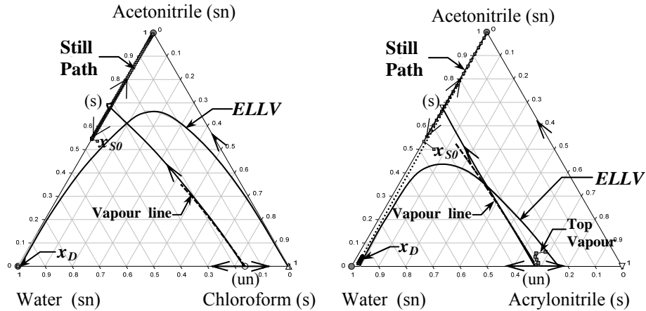
Figure 1. Residue curve map and simulation results of HABD.
