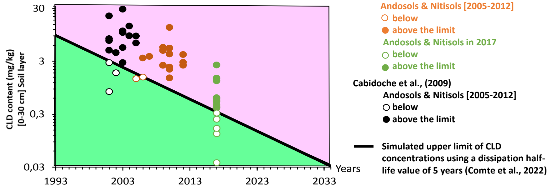
Chlordecone concentrations in soils: on-field measurements versus simulated upper limit based on a dissipation half-life of 5 years
