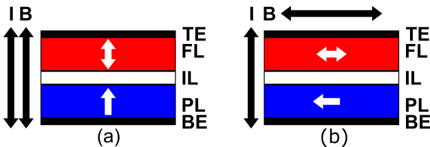
Fig. 1. Perpendicular MTJ (a) and in-plane MTJ (b). The direction of the switching current ( I ) and magnetic field ( B ) are indicated by the black arrows. The insulating layer (IL) is located between the free layer (FL) where the magnetization can be set in one of the two directions indicated by the white arrows. The pinned layer (PL) has its magnetization fixed in one direction (under normal condition), indicated by the white arrow. Two electrodes are used on the top (TE) and bottom (BE) to access the MTJ.
