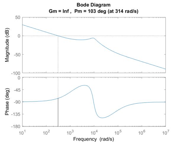
FIGURE 17. Bode diagram of open loop transfer function of controlled system for reduced scale converter tuned for a cut-off frequency of 50 Hz with gains from Table 3 (reduced scale) and parameters from Table 4, with gain margin G_m and phase margin P_m .
