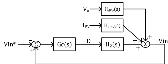
FIGURE 9. PSFB input voltage control diagram, with disturbances V_o and I_{pv} .
