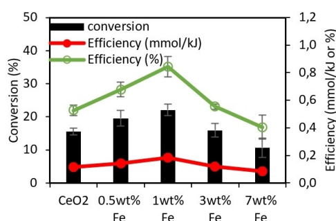
Figure 13. The effect of metal loading in the catalysts reduced at 550 °C on decomposition of ammonia. Conditions: 5% \text{NH}_3/\text{He} , 30 ml/min total flow, ambient conditions; 4 mA.
