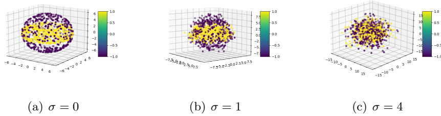
Figure 2: Data to classify. Yellow: torus, purple: sphere.
