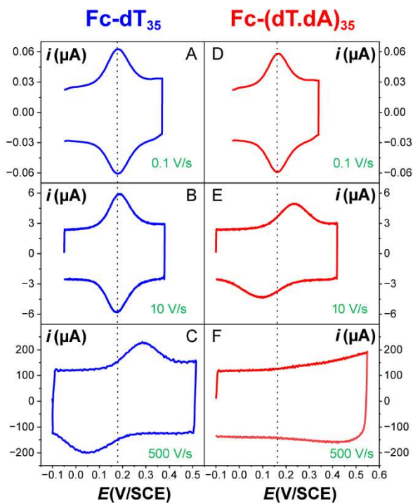
Fig. 2 Raw CV of electrode end-grafted Fc-DNA at various scan rates. (A,B,C): Fc-dT 35 chains. (D,E,F): Fc-(dT.dA) 35 chains. Chain coverage \Gamma = 5 \text{ pmol/cm}^2 . Phosphate buffered, 1 M NaClO 4 aqueous electrolyte, pH = 7. T = 25°C.
