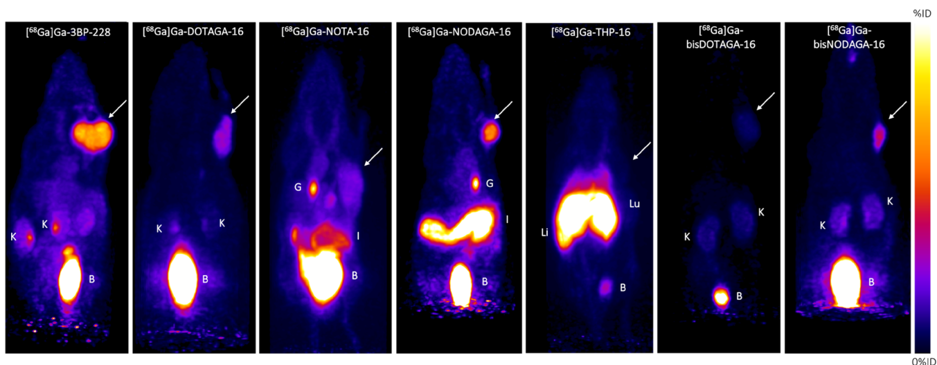
Figure 2. Maximum intensity projection (MIP) images obtained between 1.5 h and 2 h p.i. of [^{68}\text{Ga}]\text{Ga} -3BP-228, [^{68}\text{Ga}]\text{Ga} -DOTAGA-16, [^{68}\text{Ga}]\text{Ga} -NOTA-16, [^{68}\text{Ga}]\text{Ga} -NODAGA-16, [^{68}\text{Ga}]\text{Ga} -THP-16, [^{68}\text{Ga}]\text{Ga} -bisDOTAGA-16, and [^{68}\text{Ga}]\text{Ga} -bisNODAGA-16. The tumor is shown by a white arrow. Abbreviations: G, gallbladder; I, intestines; K, kidneys; B, bladder; Li, liver; Lu, lungs.
