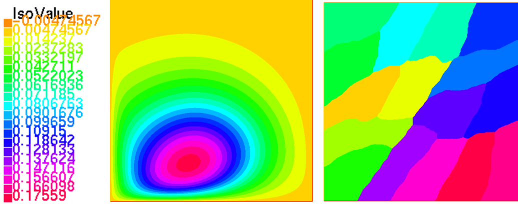
Figure 1: Left: Solution for c_0 = \nu = 0.1 . Right: Partition into N = 16 subdomains computed by Metis.
