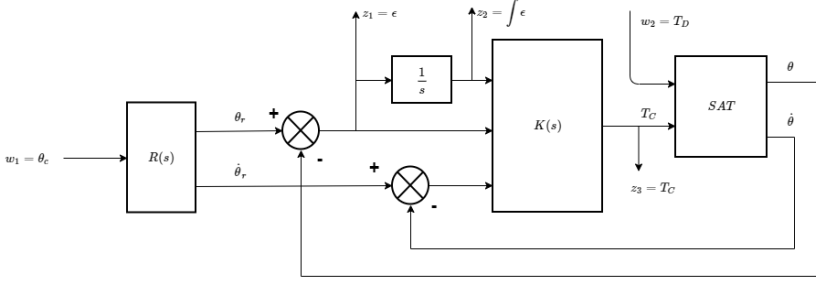
Fig. 5 H_\infty design model
