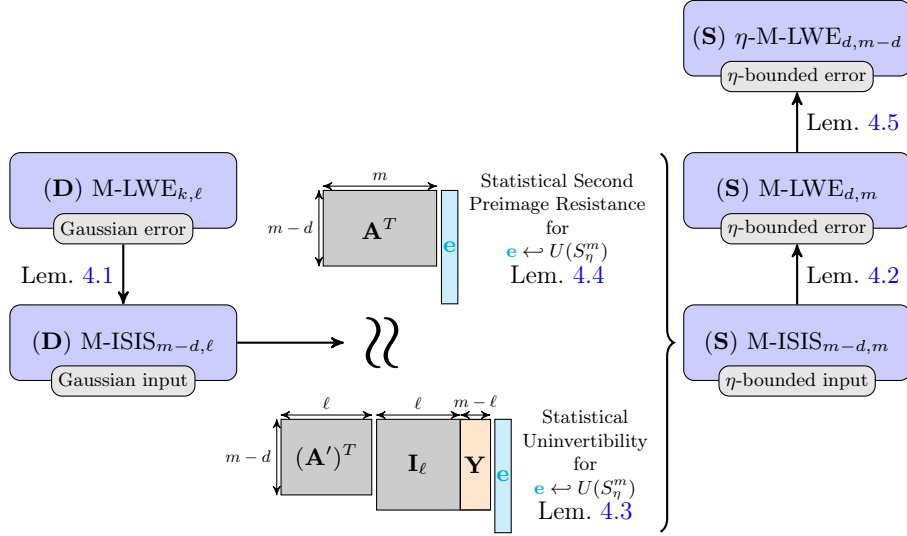
Fig. 4.1. Summary of the proof of Theorem 4.1. S denotes the search version, while D denotes the decision version. The first subscript for M-LWE denotes the rank, while the second subscript denotes the number of samples. For clarity, we removed, for both M-LWE and M-ISIS, the subscripts for the ring degree n and the modulus q as they are preserved throughout the proof. We have \ell = m - d + k .
