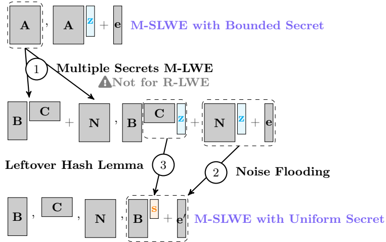
Fig. 3.1. Summary of the proof of Theorem 3.1
