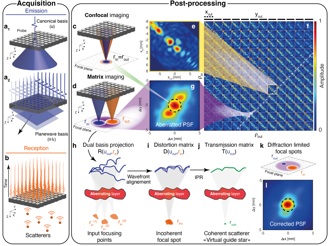
FIG. 1. 3D Ultrasound Matrix Imaging (UMI) . (a) The R -matrix can be acquired in the (a 1 ) transducer or (a 2 ) plane-wave basis in transmit and (b) recording the back-scattered wave-field on each transducer in receive. (c) Confocal imaging consists in a simultaneous focusing of waves at input and output. (d) In UMI, the input ( r_{in} ) and output ( r_{out} ) focusing points are decoupled. (e) x -cross-section of the (f) focused R -matrix. (g) UMI enables a quantification of aberrations by extracting a local RPSF (displayed here in amplitude) from each antidiagonal of R_{\rho\rho}(z) . (h) UMI then consists in a projection of the focused R -matrix in a correction (here transducer) basis at output. The resulting dual R -matrix connects each focusing point to its reflected wave-front. (i) UMI then consists in realigning those wave-fronts to isolate their distorted component from their geometrical counterpart, thereby forming the D -matrix. (j) An iterative phase reversal algorithm provides an estimator of the T -matrix between the correction basis and the mid-point of input focusing points considered in panel f. (k) The phase conjugate of the T -matrix provides a focusing law that improves the focusing process at output. (l) RPSF amplitude after the output UMI process. The ultrasound data shown in this figure corresponds to the pork chop experiment at depth z = 40 mm.
