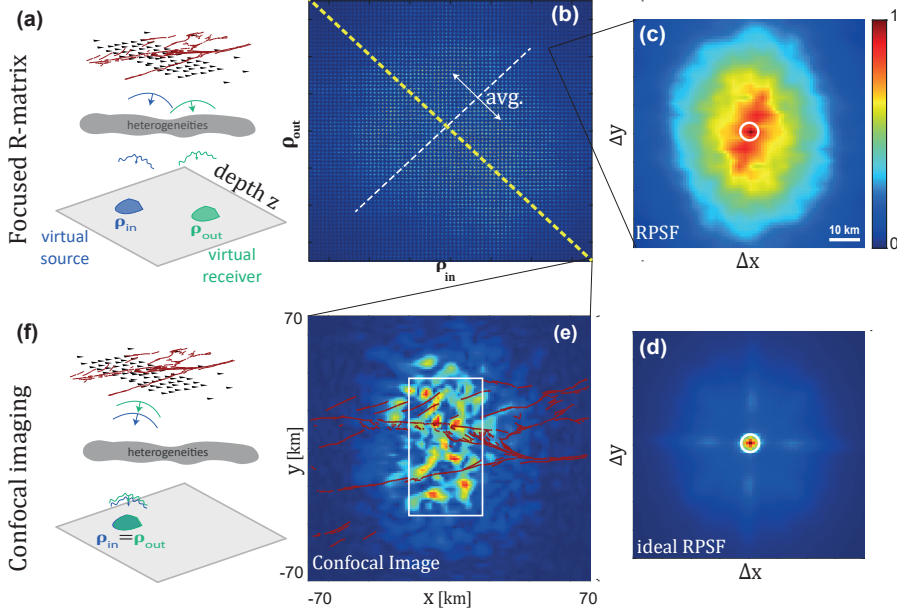
FIG. 2: Focused reflection matrix. (a) The response matrix \mathbf{K} is projected onto a focused basis at each depth z (Eq. 7), thereby synthesizing a set of virtual sources ( \boldsymbol{\rho}_{\text{in}} ) and receivers ( \boldsymbol{\rho}_{\text{out}} ) scanning laterally the field-of-view. In presence of fluctuations in the seismic velocity, focused waves are distorted while travelling from the surface to the plane, thereby enlarging and distorting the virtual geophones. (b) This effect gives rise to a off-diagonal spreading of backscattered energy in the focused reflection matrix \mathbf{R}_{\rho\rho}(z) shown here at depth z = 25 km. (c) The corresponding intensity profile, averaged over whole the field-of-view, provides the so-called RPSF I (Eq. 12). The white circle represents the diffraction-limited transverse resolution ( \delta\rho_0 \sim 6 km) at the considered depth. (d) The ideal RPSF that would be obtained in absence of aberrations is shown for comparison (e) Confocal image \mathcal{I} (Eq. 10) built from the diagonal of \mathbf{R}_{\rho\rho} . The white box represents the dimensions of the rectangular array of geophones and the red lines represent the NAFZ fault traces at the surface. (f) The confocal image corresponds to a simultaneous focusing process at input and output ( \mathbf{r}_{\text{in}} = \mathbf{r}_{\text{out}} ). In panels (b)-(e), the color scale refers to the scattering intensity. It is normalized by the maximum value of the scattering energy at the considered depth.
