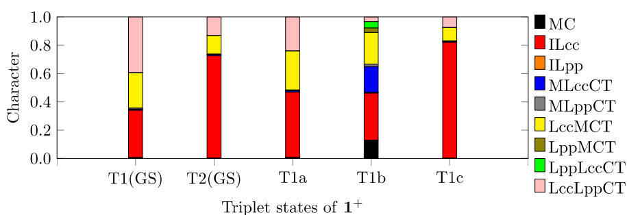
Figure 9. Nature of the T_1 and T_2 states at Franck-Condon geometry of 1^+ , namely T_1(\text{GS}) and T_2(\text{GS}) , and of T_{1a} , T_{1b} and T_{1c} at their optimized geometry. Subscript CC and PP stands for the biphenyl ligand and diphosphine ligand, respectively.
