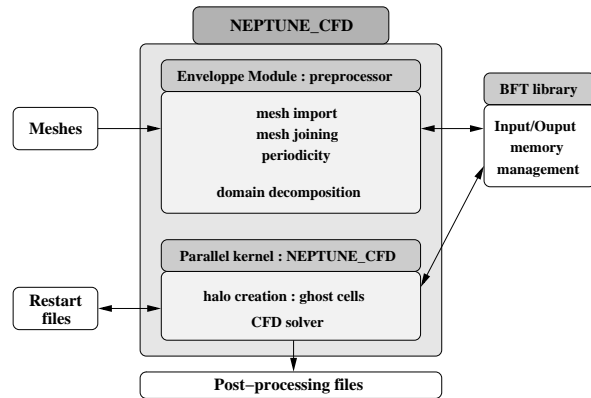
Figure 1: NEPTUNE_CFD modules.
