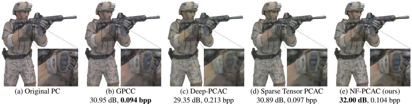
Fig. 4: Visual results of all the different architectures tested
