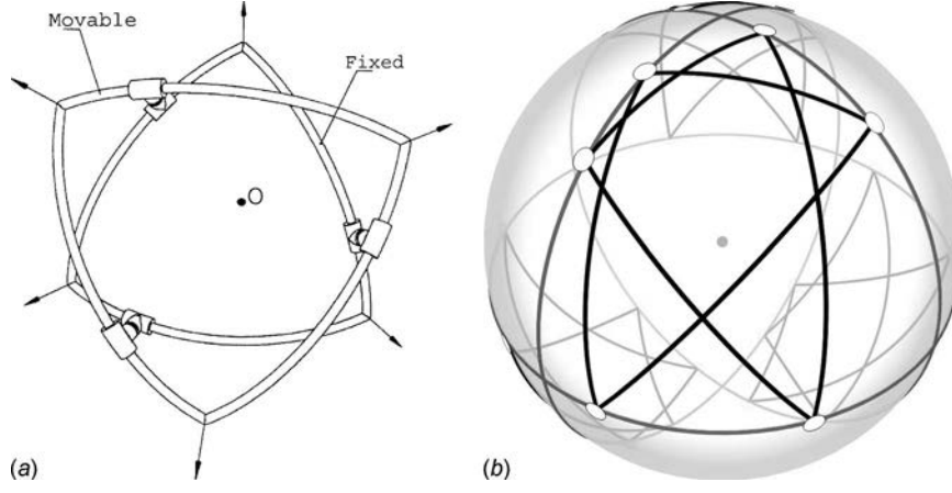
Fig. 4 Spherical double triangular manipulator
