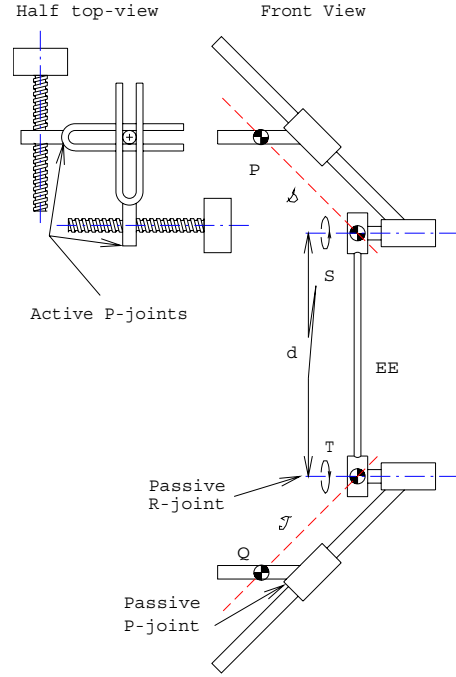
Fig. 3 Two screw actuators for double basal actuation
