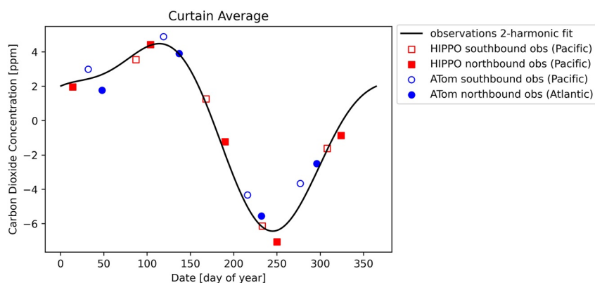
Figure 2. Two-harmonic fit to detrended average carbon dioxide concentration in ppm as a function of day of year for HIPPO and ATom flight campaigns in the atmospheric curtain between 20°N and 90°N in latitude and between 1,000 and 300 hPa in pressure. The points are found by filtering, detrending, interpolating and extrapolating to get a full altitude and latitude slice, then taking a pressure and cosine of latitude-weighted average. The black line is the average of all fits to individual latitude-pressure bins with the annual mean removed. The direction of flight (southbound or northbound) is shown with filled and unfilled symbols because southbound flights occurred 2–3 weeks earlier than northbound flights.
