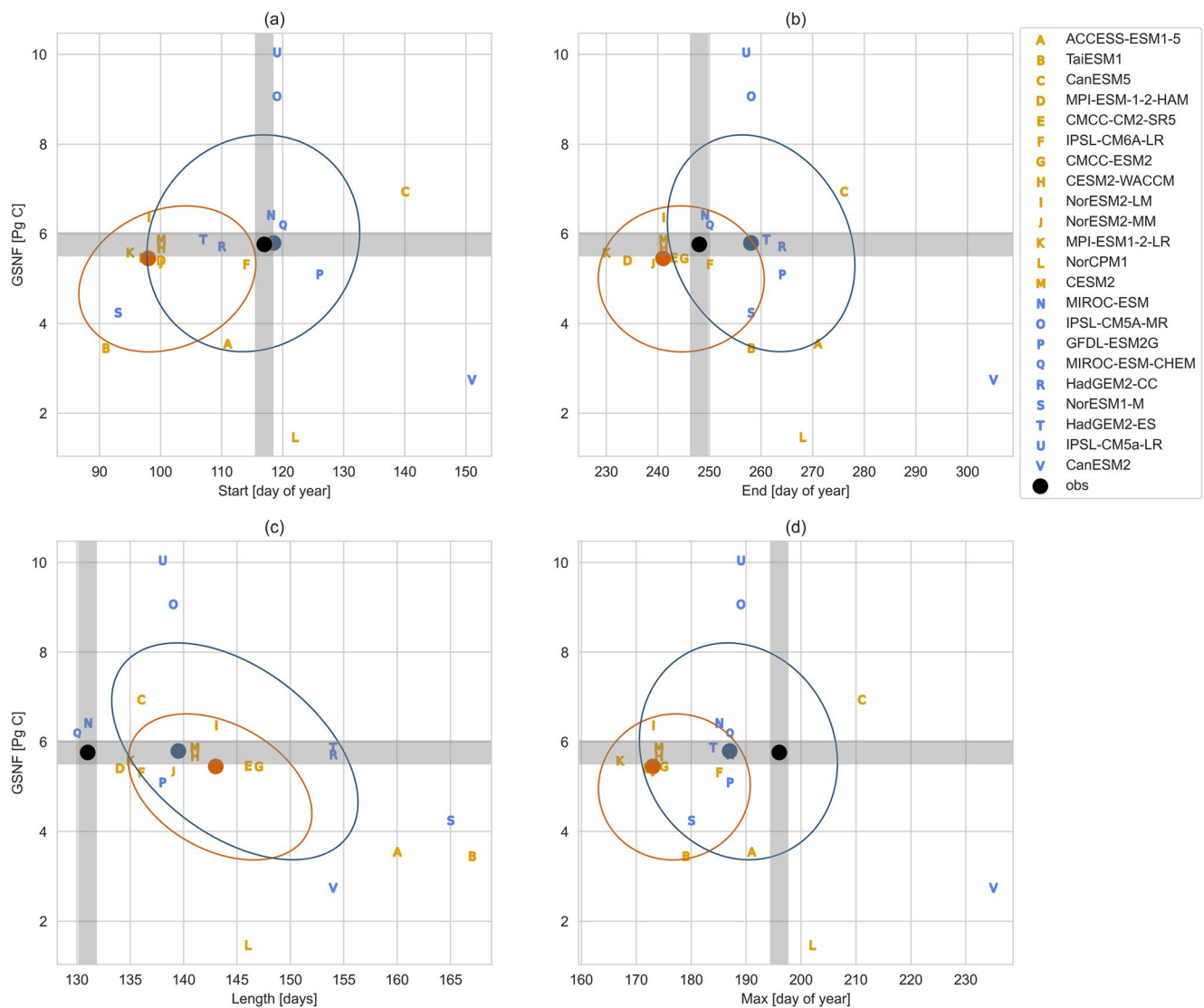
Figure 5. Growing season net flux plotted against the (a) start of the season, defined to be the first day when the seasonal component of atmospheric CO 2 is decreasing (seasonal component of flux changes from positive to negative), (b) end of the season, defined to be the last day when the seasonal component of atmospheric CO 2 is decreasing (seasonal component of flux changes from negative to positive), (c) length of the season, and (d) max of season, defined to be the day when flux is most negative. The black point is the number inferred from the observations with gray lines showing uncertainty. Coupled Model Intercomparison Project phase 5 (CMIP5) models are shown in blue and Coupled Model Intercomparison Project phase 6 (CMIP6) models are shown in orange. The blue and orange points are the multi-model mean for the CMIP5 and CMIP6 ensembles, respectively. The surrounding ellipses show the covariance to one standard deviation. Only models where gross primary productivity, heterotrophic respiration and net primary productivity output were available are included.
