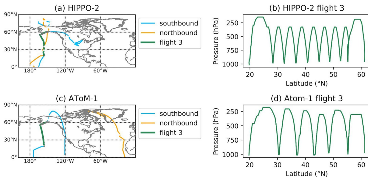
Figure 1. Flight paths for (a) HIPPO-2, which flew over the remote Pacific in November 2009, and (c) ATom-1, which flew over the Pacific and Atlantic in August 2016. All other campaigns followed similar flight paths. Flight path with continuous vertical profiling for flight 3, which flew from Anchorage, AK to Kona, HI for (b) HIPPO-2 and (d) ATom-1. All other flights flew a similar path.
