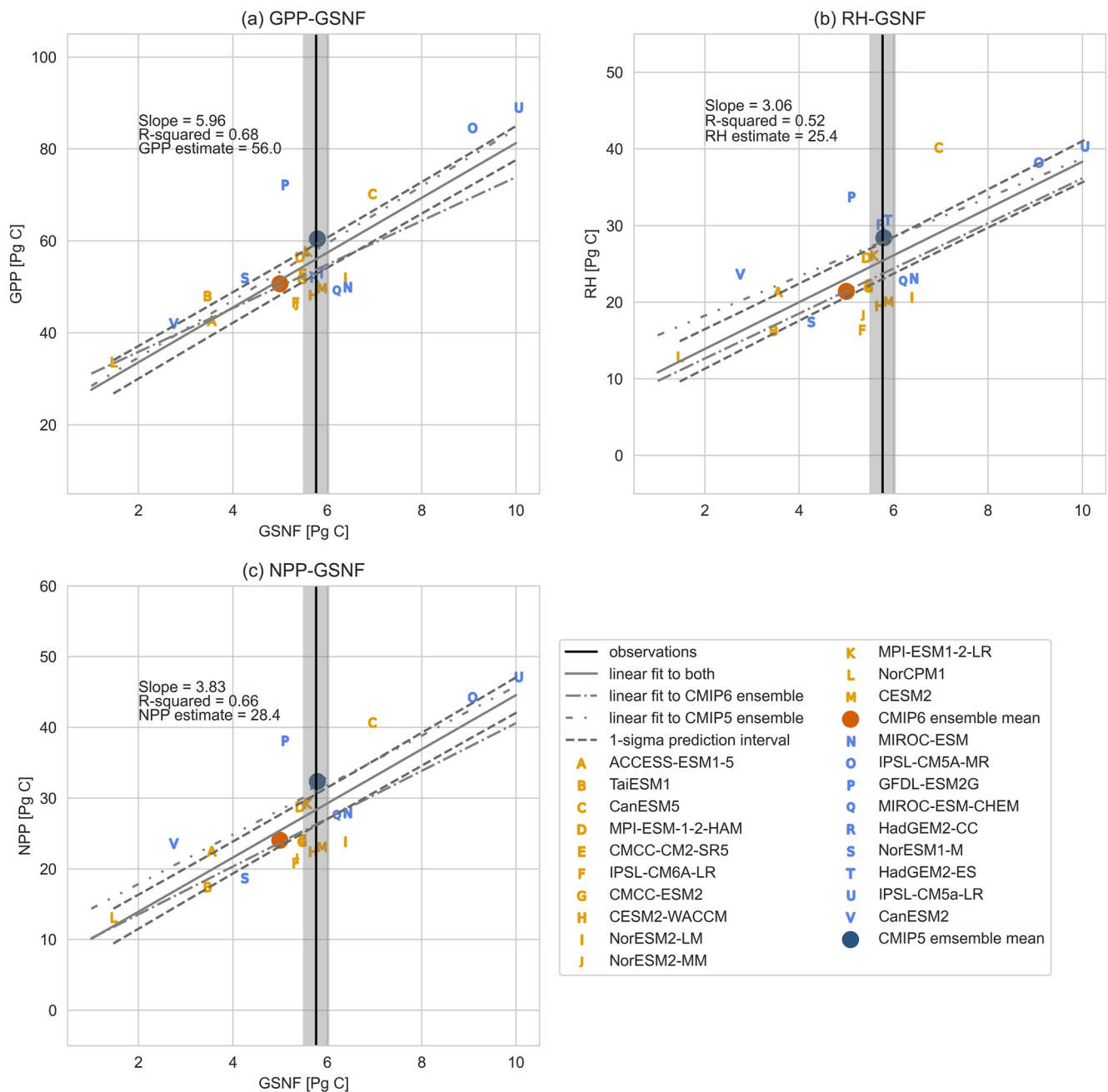
Figure 7. Growing season net flux (GSNF) plotted as a function of (a) integrated gross primary productivity (GPP) and (b) integrated heterotrophic respiration (RH), and (c) integrated net primary productivity (NPP) for the Coupled Model Intercomparison Project phase 5 (CMIP5) and Coupled Model Intercomparison Project phase 6 (CMIP6) models. The estimated GSNF from the HIPPO and AToM observations is shown in gray, CMIP5 models are shown in blue, and CMIP6 models are shown in orange. Only models where GPP, RH, and NPP data were available were included.
