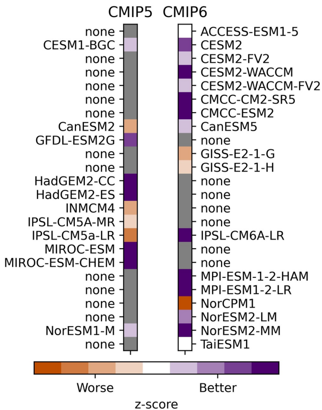
Figure 6. Coupled Model Intercomparison Project phase 5 and Coupled Model Intercomparison Project phase 6 model absolute values of z-score calculated for all models. The color gray and the label, none have been used when one generation of a model is not used or not existent.
