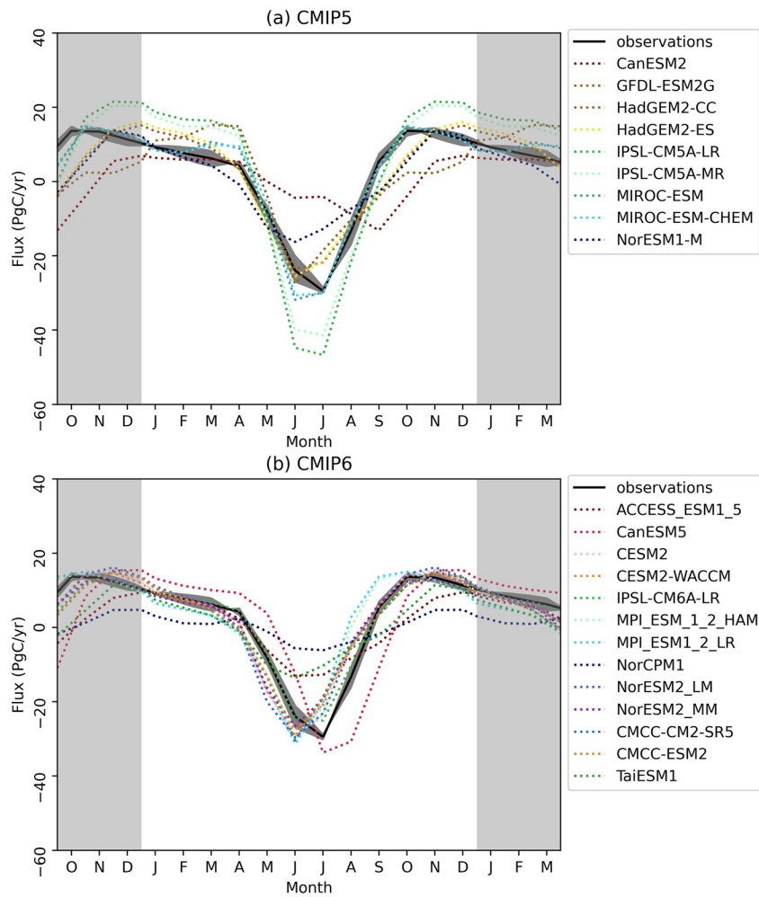
Figure 4. Corrected flux estimated from the HIPPO and ATom campaigns in comparison to area-weighted average NBP in the same domain from the (a) Coupled Model Intercomparison Project phase 5 (CMIP5) and (b) Coupled Model Intercomparison Project phase 6 (CMIP6) models. The bias corrected observation error is the standard deviation between correction using the three different inverse models. While the spread in magnitude and timing of the flux in the CMIP6 models is smaller than that of the CMIP5 models, there is still disagreement between the models.
