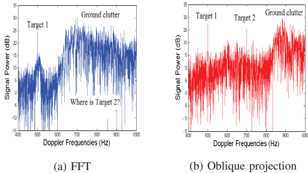
Fig. 4. FFT and oblique projection for real clutter data
