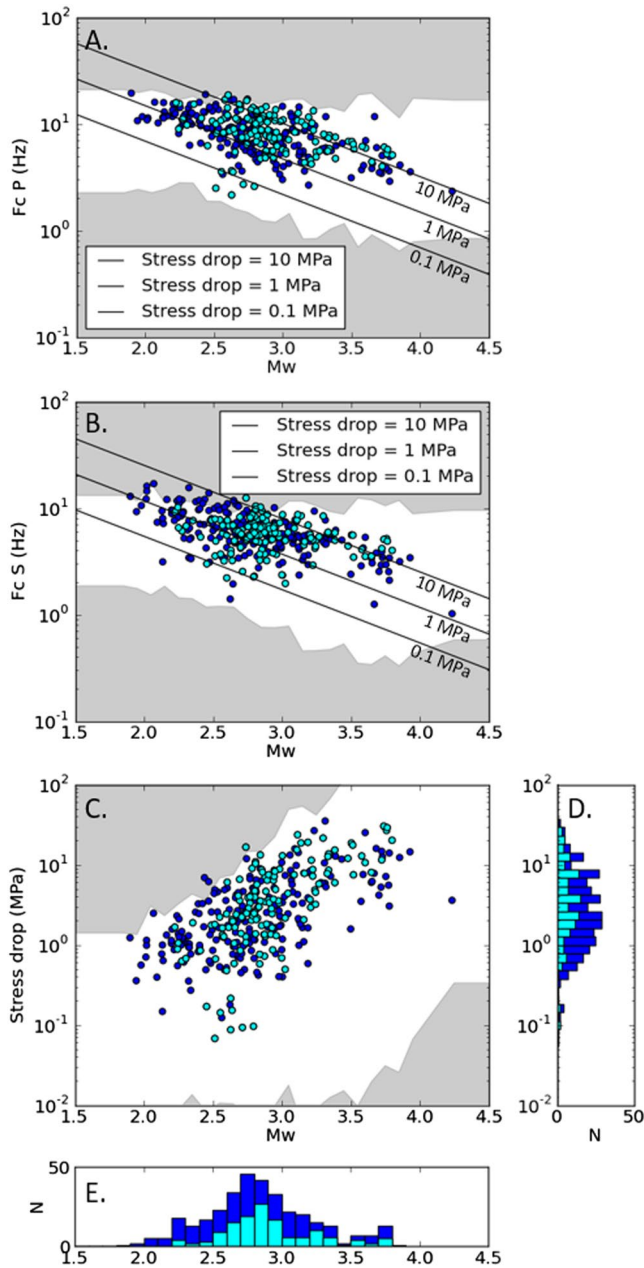
Figure 4. Panels (a)–(c) show source properties (corner frequencies inferred from P -waves and S -waves, stress drop) as a function of moment magnitude. Panels (d) and (e) show the distribution of stress drops and magnitudes respectively. Light blue represents repeaters and dark blue represents non-repeaters. The gray shaded areas show for a given magnitude the median upper and lower frequency limits between which corner frequencies can be resolved.
