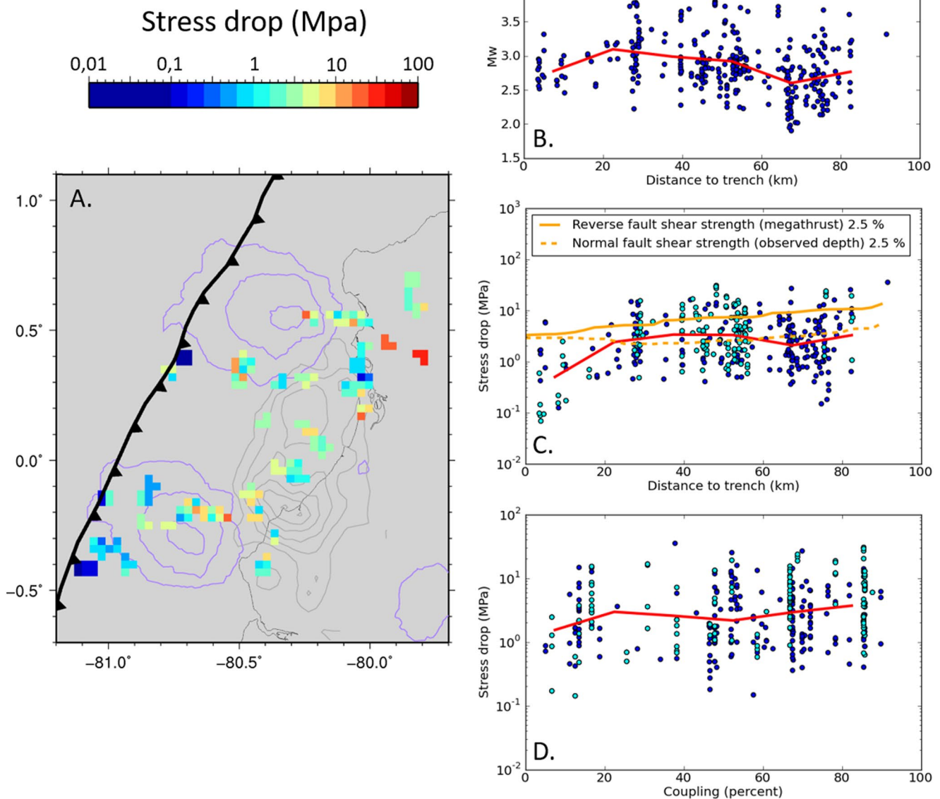
Figure 7. Spatial distribution of stress drop. (a) shows a map of all stress drops calculated, with colors representing their logarithm. The purple lines are the 20 cm contours of the afterslip (Rolandone et al., 2018), while the gray lines are the 1 m contours of the Pedernales rupture (Nocquet et al., 2017). (b) Shows the magnitude of events with full source properties as a function of distance to the trench. (c) Shows stress drop as a function of distance from the trench, with the orange lines showing the expected shear strength based on earthquake depth, and the depth of the interface (Hayes et al., 2012). (d) shows the relationship of stress drops to coupling. In b, c, and d, the red line is the median.
