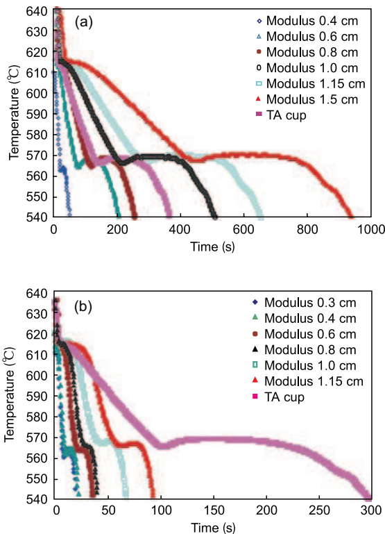
Fig. 3: Cooling curves for alloy 2 obtained for cylindrical castings of different modulus and standard TA cup (a) sand mould; (b) metallic mould
