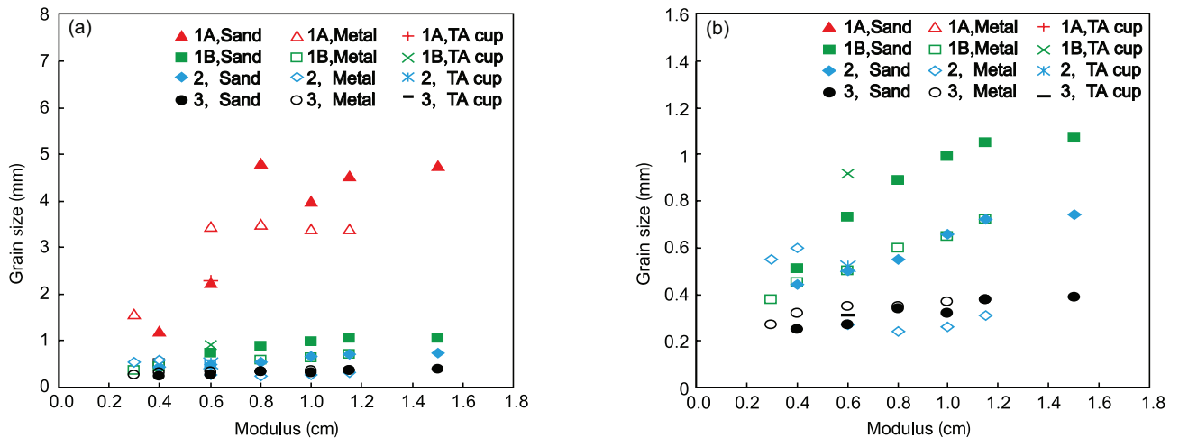
Fig. 5: Grain size values vs thermal modulus (a) and an enlargement for small grain sizes (b) (The data for TA cups are also included)
