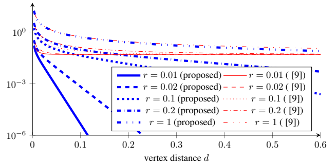
Fig. 2: Edge weight upper bounds for both [9] and our proposed approach, and for varying ranges of the variogram.
