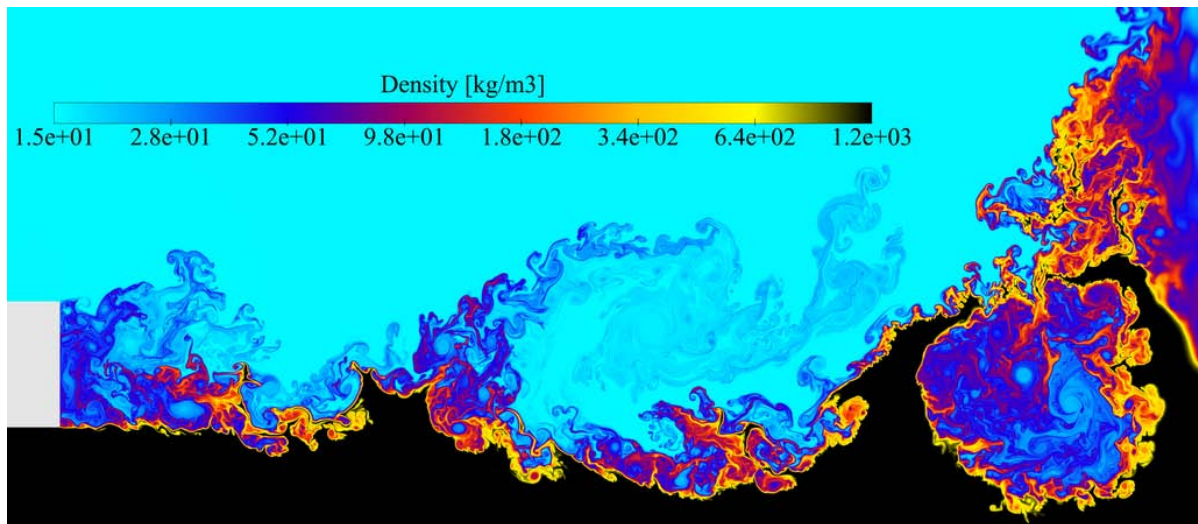
Figure 4: Density field, ranging from 15 kg.m -3 (blue) to 1200 kg.m -3 (black) using a logarithmic scale.
