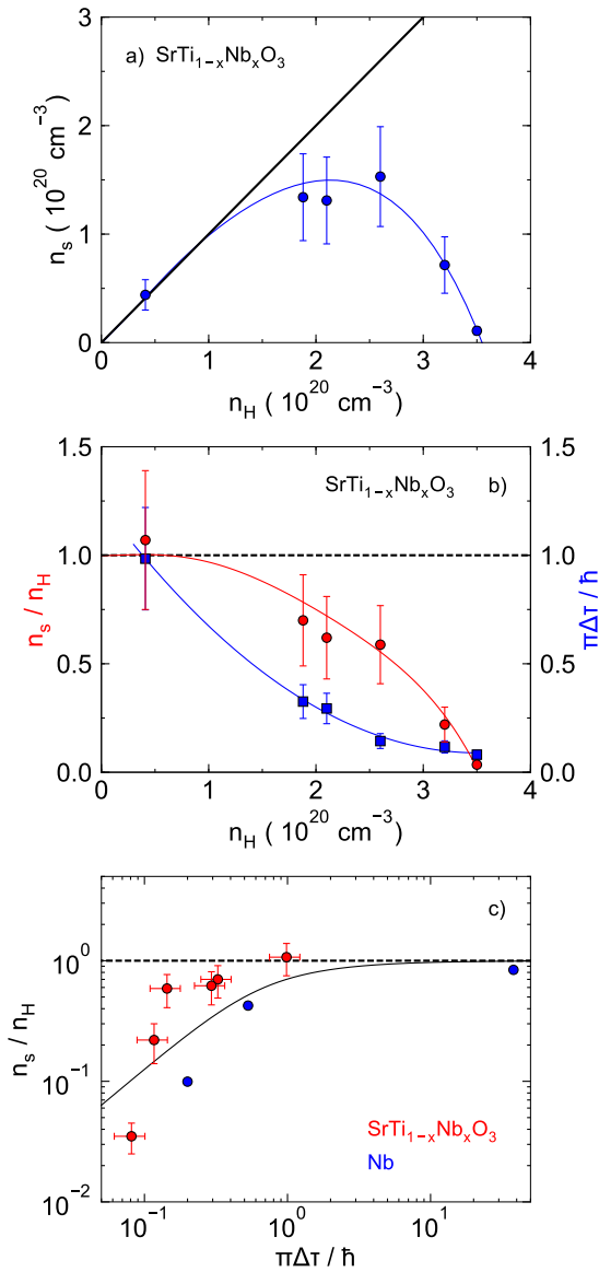
FIG. 6. a : Evolution of superfluid density as a function of carrier density. The straight line represents n_s = n_H . b : The ratio of superfluid density over normal-state carrier density (red discs) compared to the product of the scattering time and the superconducting gap (blue squares) as a function of doping. Lines are guides to the eye. c : The evolution of superfluid density in Nb (blue squares[43, 54, 55]) and in Nb-doped SrTiO 3 (red discs). The continuous black line is the analytic solution of the Ferrell Glover Tinkham sum rule Eq.7.
