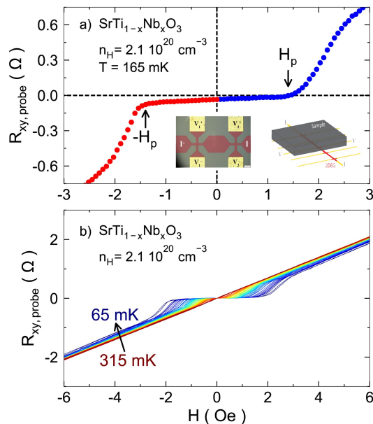
FIG. 1. a : Typical field dependence of the Hall resistivity of a microprobe with a superconducting sample above. The measured signal, directly proportional to the local magnetic field, suddenly rises when the first vortex penetrates the sample. The sharpness indicates the absence of surface-barrier effects or gradual vortex leak from sample corners[27]. The inset shows, in false colors, a picture of the array of Hall microprobes used for this experiment and a scheme of how a sample is mounted on the array of probes. b : Raw data for the n_H = 2.1 \cdot 10^{20} \text{ cm}^{-3} sample at different temperatures.
