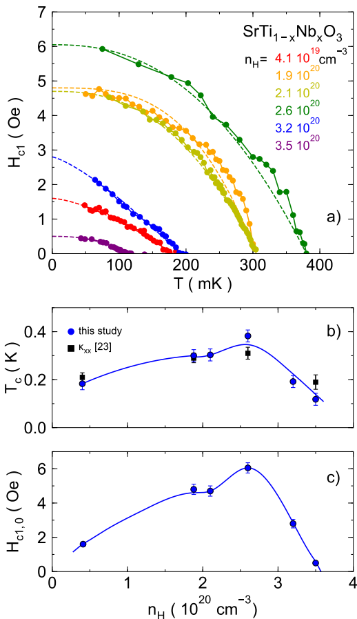
FIG. 3. a: Lower critical field vs temperature for all six samples deduced from H_p and geometrical correction of the demagnetization field. b: Doping dependence of the critical temperature determined by Hall probe magnetometry (blue disks) and thermal conductivity (black squares)[33], the blue line is a guide to the eye. c: Doping dependence of H_{c1} , the blue line is a guide to the eye.
