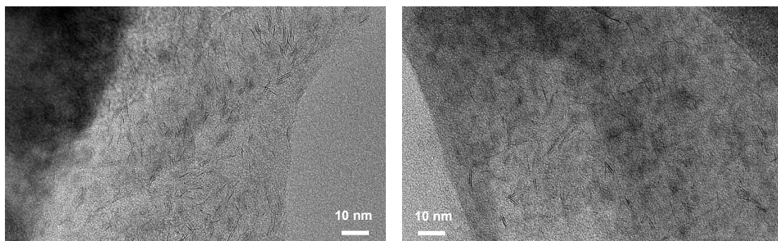
Figure 16. Representative TEM images of model P-doped MoS 2 catalysts supported on the M(10 \bar{1} 0) plane of \alpha -Al 2 O 3 . Left: low P-content (initial P/Mo = 0.11), Right: high P-content (initial P/Mo = 0.57)
