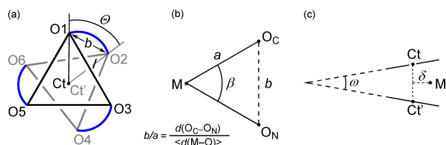
Figure 8. Graphical definitions of the stereochemical parameters for the octahedral/trigonal prismatic geometries of [ML_3] complexes, where L is a bidentate chelate (shown as an arc of a circle in blue). M is the metal cation, Ct and Ct' are the centroids of oxygen donors located in the same plane when the complex is viewed along its pseudo- C_3 symmetry axis. (a) Trigonal twist angle \theta ( \theta = 60^\circ for an ideal OC or 0^\circ for an ideal TPR); (b) bite angle \beta and normalized bite b/a ; (c) tilt angle \omega between both trigonal faces (O1,O3,O5) and (O2,O4,O6), and lateral metal displacement \delta from the Ct–Ct' axis.
