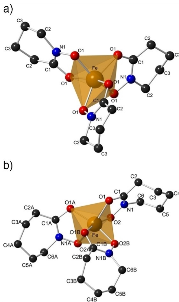
Figure 9. Pictorial representations of the coordination polyhedra of (a) [\text{Fe}(\text{PIPO})_3] and (b) [\text{Fe}(\text{AZEPO})_3] .
