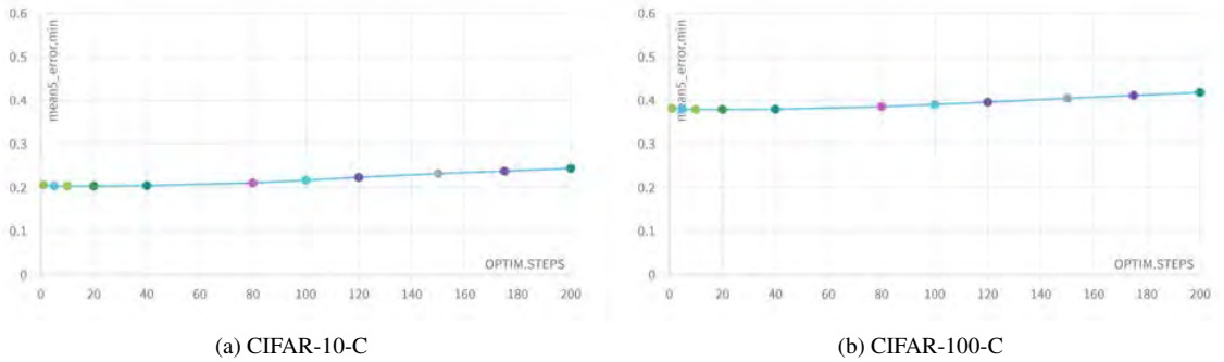
Figure 2. Online mean error along all corruptions at severity 5 for different number of learning steps of TTAwPCA.
