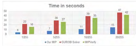
Figure 3: Computational Time for robustness problems averaged over 100 instances according to the intensity of the attack (maximum disturbance allowed in infinite norm)
