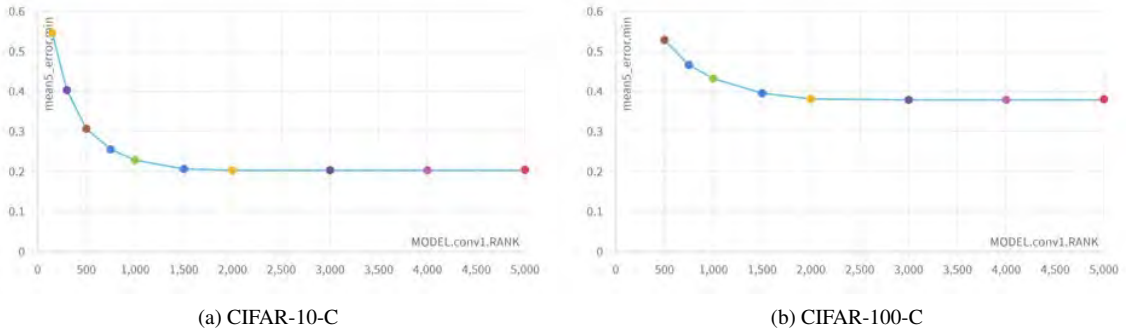
Figure 1. Episodic mean error along all corruptions at severity 5 for different rank of the PCA of TTAwPCA.
