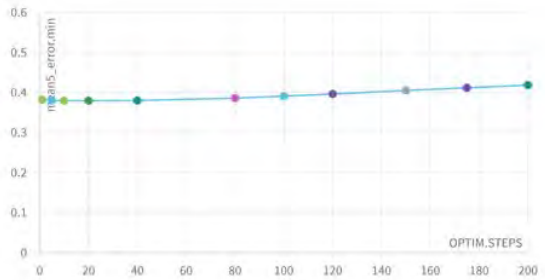
(b) CIFAR-100-C
