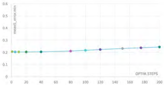
(a) CIFAR-10-C
