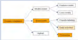
Taxonomy of DA methods (from Ramponi and Plank, 2020)
