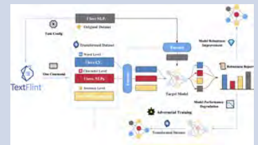
Example of TextFlint (https://github.com/confianceai/textflint)
