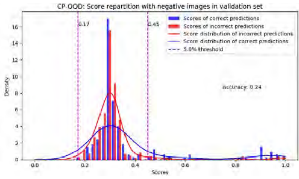
Fig 5: Correct and incorrect prediction distributions for CP-OOD on the negative validation dataset
