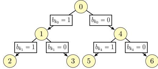
Figure 1: Separation step in a binary search tree: each node corresponding to the optimization problem \mathcal{P}^{(n)} , is divided into two children nodes obtaining by constraining one variable to be zero or non-zero.
