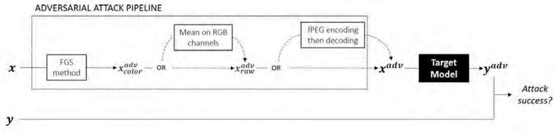
Figure 1: The robustness evaluation pipeline of a target model
