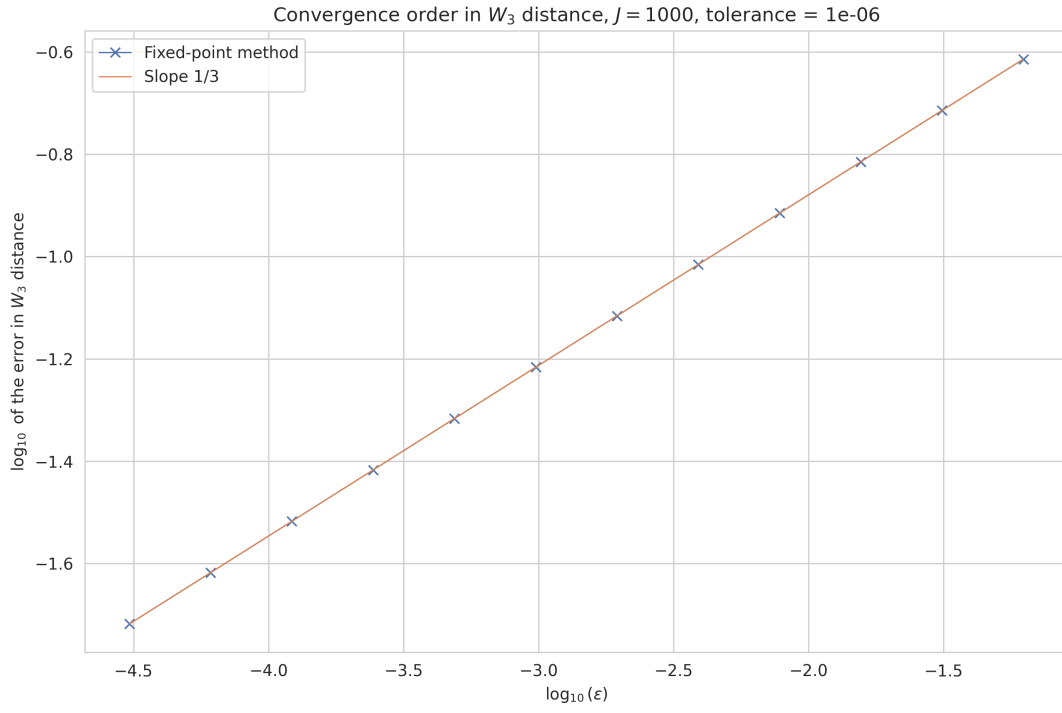
Figure 5: O(\epsilon^{1/3}) convergence in W_3 distance of \rho^\epsilon towards \delta_0 , W(x) = |x|^3 . The initial density is the centered Gaussian 2\sqrt{\frac{5}{\pi}}e^{-20x^2} .
