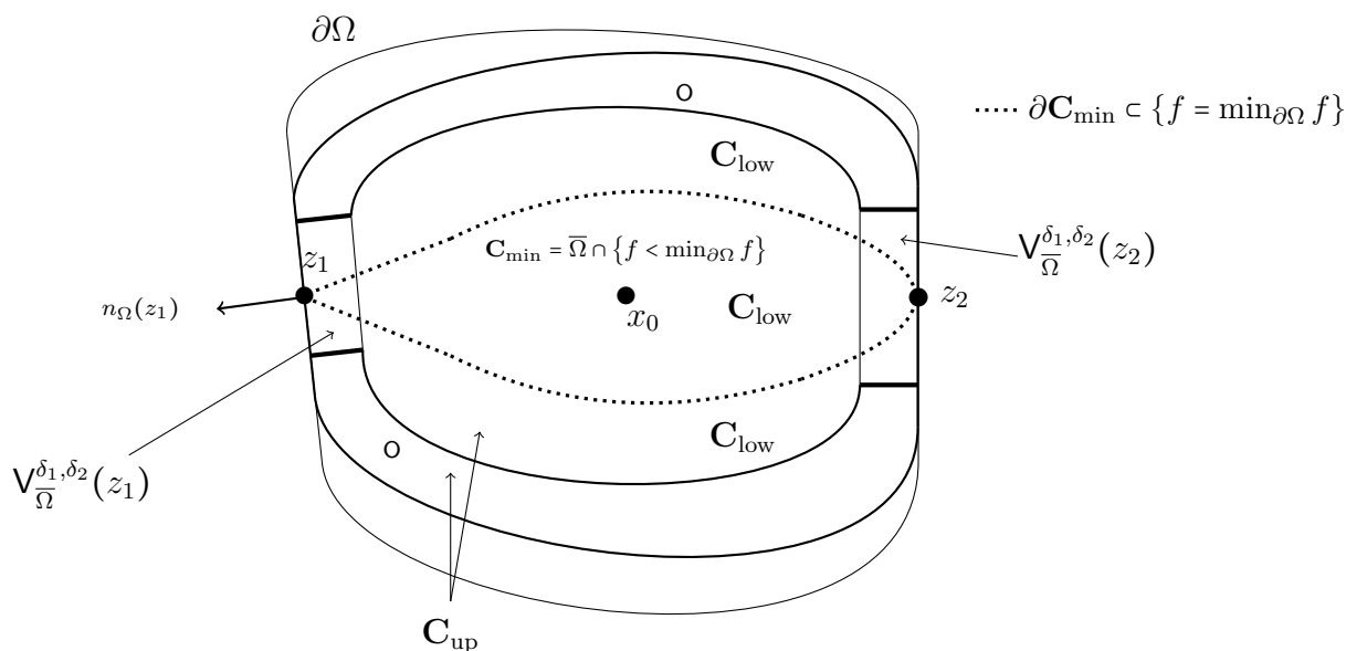
FIGURE 5.1. Schematic representation of \mathbf{C}_{\text{low}} , \mathbf{C}_{\text{up}} , and \mathbf{O} (see Proposition 20). On the figure, \partial\mathbf{C}_{\text{min}} \cap \partial\Omega = \{z_1, z_2\} with \nabla f(z_1) = 0 and |\nabla f(z_2)| \neq 0 .
