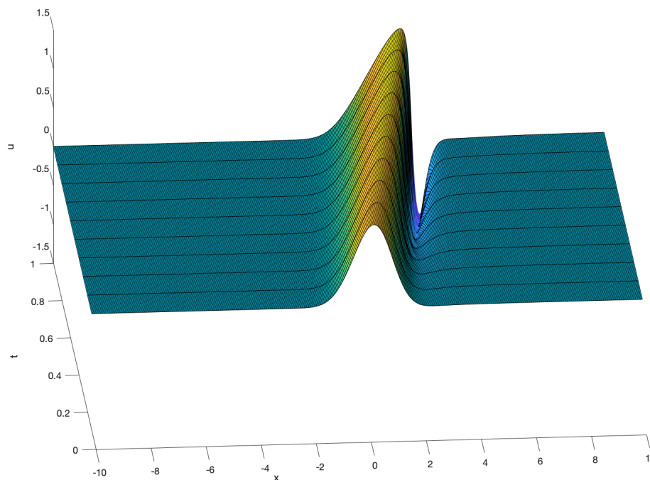
FIGURE 4. Test 3. Numerical solutions of the morphodynamics model (1) with initial condition (30) for t \in (0.1, 1)
