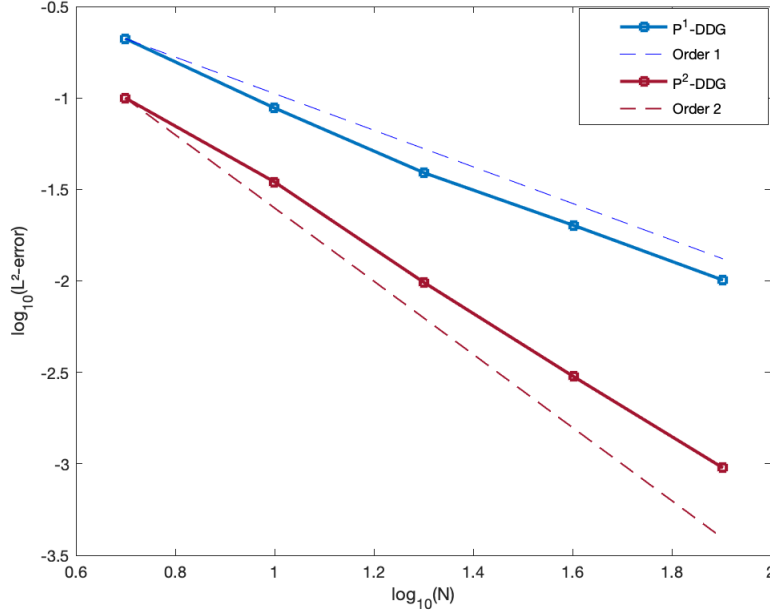
FIGURE 1. Test 1: Convergence curves for k = 1 (solid blue line) and k = 2 (solid red line). Dashed lines represent slopes of order 1 (in blue) and of order 2 (in red).
