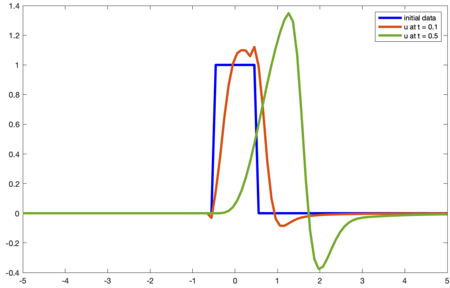
FIGURE 2. Test 2: Numerical solutions of (28) with \eta = 1, \varepsilon = 0.01 and N = 100
