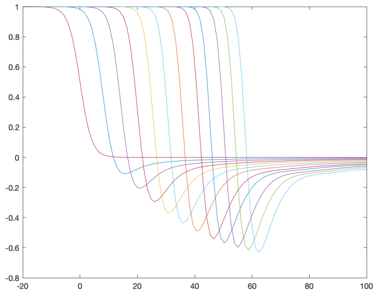
FIGURE 3. Test 3: Numerical solutions for different times of (1) with the initial data (29)
