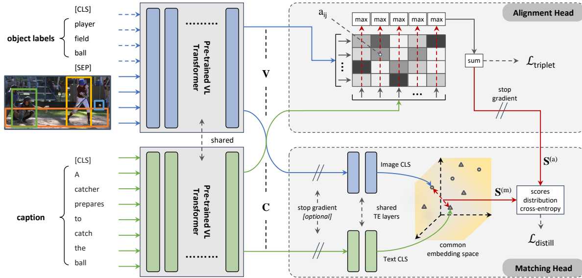
Figure 6. Overview of the ALADIN architecture [57].
