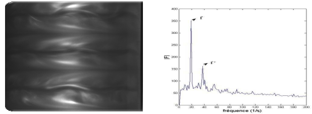
Figure 2: (Left) Visualization of modulated wavy vortex flow (Re=2000). (Right) Spectrum with two peaks related to modulated waves
