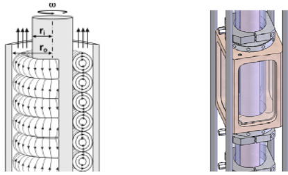
Figure 1: (Left) Geometry of Taylor-Couette vortices – (Right) Sketch of experimental device.
