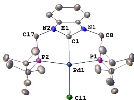
Figure 2. Structure of [PdCl(PC sp 3 H 2 P)] ( 3 ) in 3 · 2 C 6 H 6 with H atoms except PdCl–H1 omitted for clarity. Thermal ellipsoids are shown at 50% probability. Selected bond lengths [Å] and angles [°]: Pd1–C1 2.086(2), Pd1–Cl1 2.4561(6), Pd1–P1 2.3288(6), Pd1–P2 2.3219(6), C1–N1 1.448(3), C1–N2 1.452(3); N1–C1–N2 102.19(17), N1–C1–Pd1 114.58(14), N2–C1–Pd1 115.19(14), C1–Pd1–Cl1 176.89(6), P1–Pd1–P2 163.34(2), C1–Pd1–P1 82.24(6), C1–Pd1–P2 82.13(6), P1–Pd1–Cl1 98.20(2), P2–Pd1–Cl1 97.72(2), N1–C1–N2 102.2(2).
