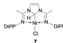
Scheme 5. The Ni^{II} N^{imino}C_{sp^3}H^{imino} pincer complex 7 . [95]
