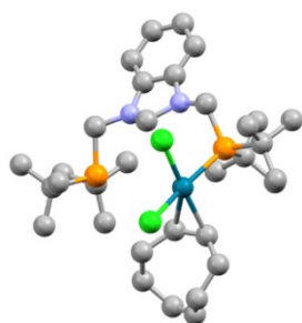
Figure 5. Computed structure of the \text{Pd}^{\text{II}} intermediate I1, hydrogen atoms are omitted for clarity.
