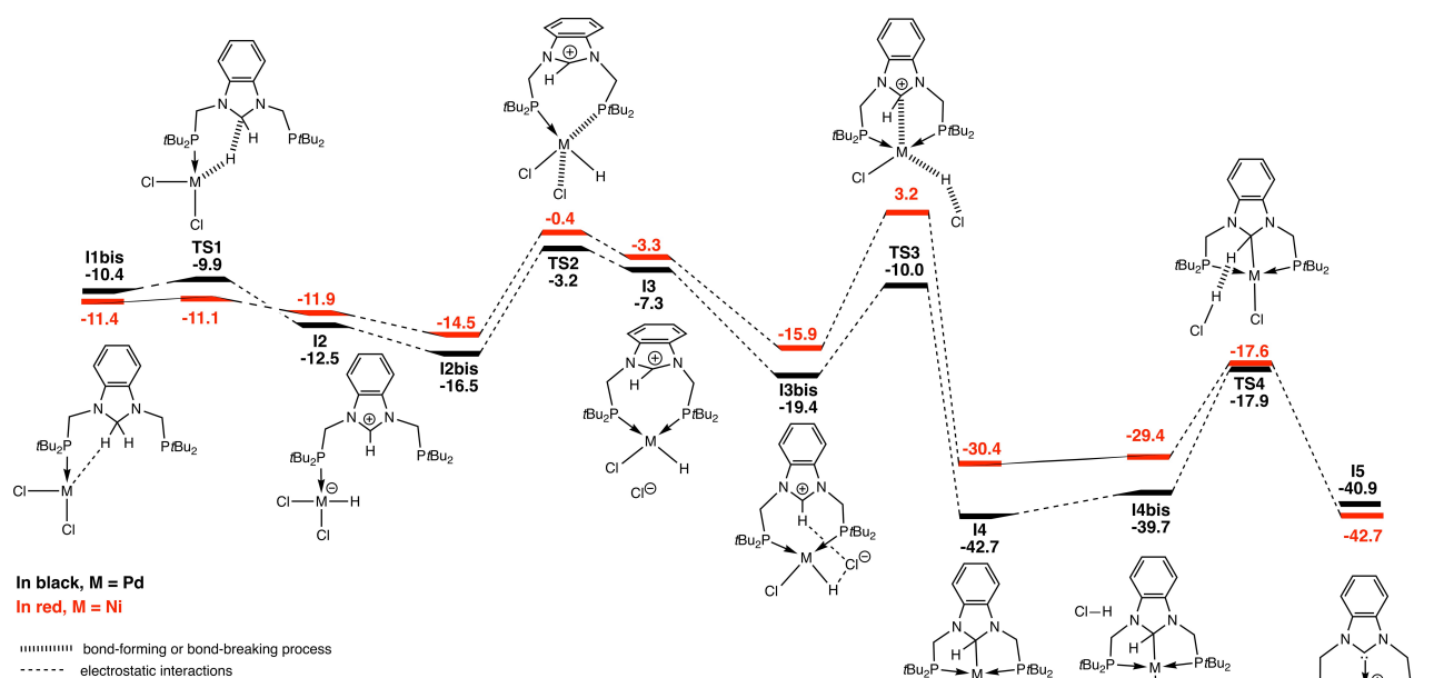
Figure 4. Mechanism of the \text{CH}_2 double activation with energies in \text{kcal}\cdot\text{mol}^{-1} .
