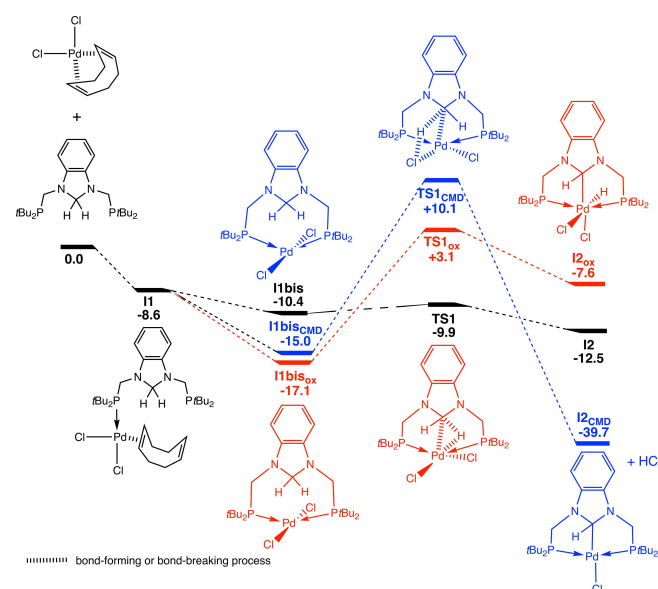
Figure 6. Alternative mechanisms for the \text{CH}_2 double activation with energies in \text{kcal}\cdot\text{mol}^{-1} . the mechanism proposed in Figure 4 is in black, the mechanism for the oxidative addition in red and the CMD mechanism is in blue.
