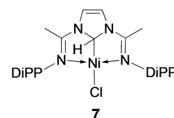
Scheme 5. The Ni^{II} N^{imino}C_{sp^3}H^{imino} pincer complex 7 . [95]
