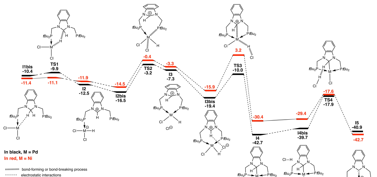
Figure 4. Mechanism of the CH 2 double activation with energies in kcal·mol -1 .
