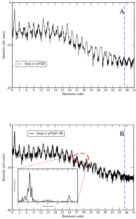
Fig. 3 A: HHG spectrum of the argon atom using I = 3 \times 10^{14} W/cm 2 and \lambda_0 = 800 nm with a 4aug-cc-pVQZ basis set. B: the same as for A but with a 4aug-cc-pVQZ+5K basis set. Ionisation is taken into account using d_0 = 28 a.u. and d_1 = 0.1 a.u.. Inset in panel B shows the non-logarithmic HHG spectrum at minimum.
