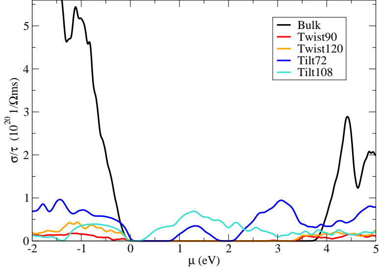
Figure 6: \sigma/\tau as a function of the chemical potential for the tilt and twist GBs structures studied.
