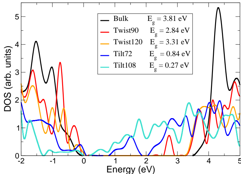
Figure 4: DOS and energy gaps of the tilt and twist GBs studied.
