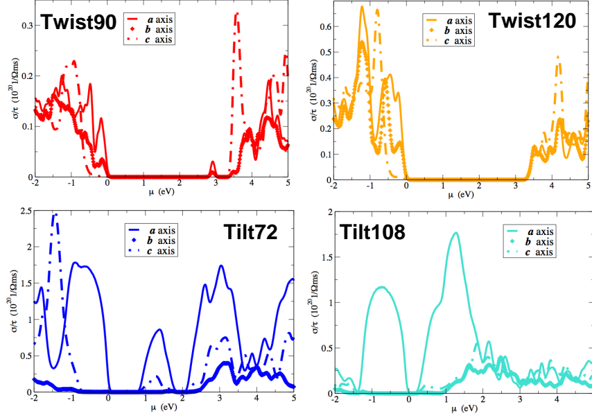
Figure 7: \sigma/\tau projected along a , b and c axis as a function of the chemical potential for the tilt and twist GBs structures studied.
