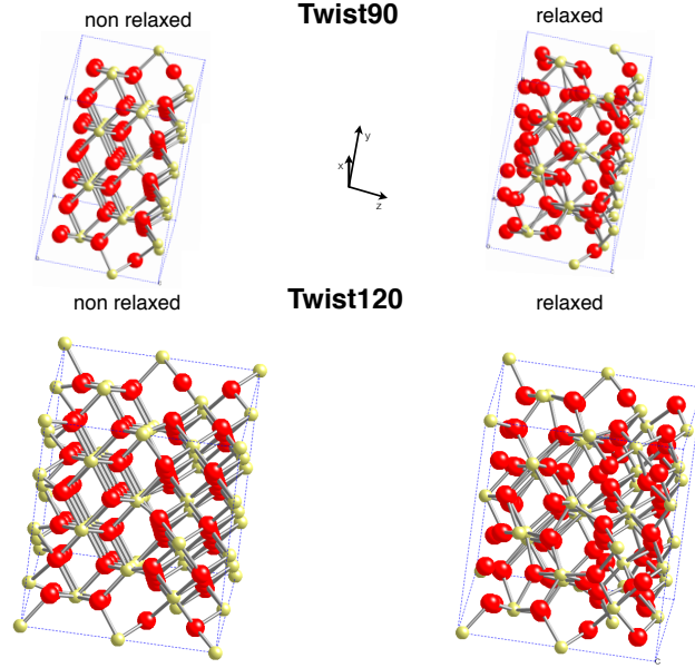
Figure 3: Twist90 and Twist120 are shown before and after geometrical relaxation.
