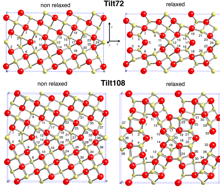
Figure 2: Tilt72 and Tilt108 are shown before and after geometrical relaxation.
