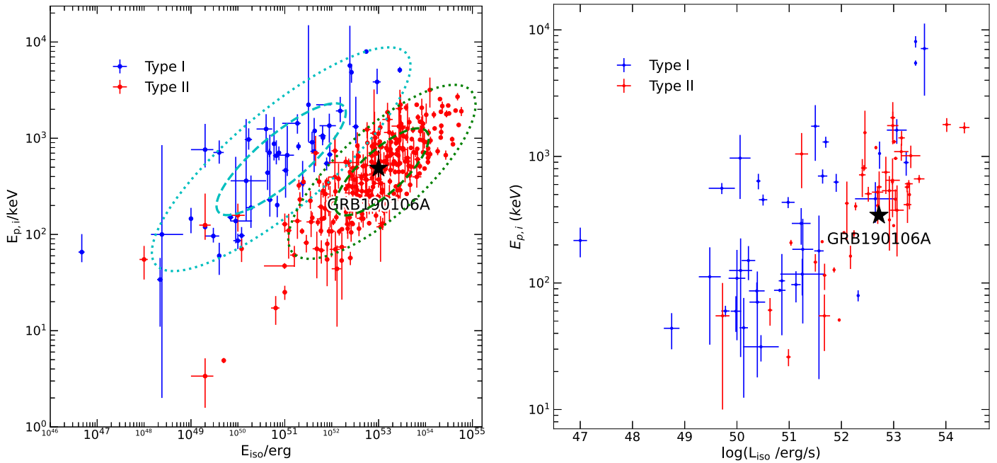
Figure 9. Left panel: Amati diagram of GRB 190106A (black star). Dashed and dotted lines represent 1\sigma and 2\sigma confidence levels, respectively. The ellipses colored in cyan and green represent type I and type II burst confidence, respectively. The data points for type I and type II GRBs are taken from Minaev & Pozanenko (2020). The burst lies within the 1\sigma confidence region of type II bursts, consistent with the E_p - E_{\text{iso}} correlation. Right panel: Yonetoku diagram of GRB 190106A (black star). The data points for type I and type II GRBs are taken from Nava et al. (2012) and Zitouni et al. (2022).
