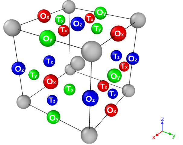
Figure 1: Body-centered orthorhombic cell with iron atoms (grey), octahedral interstitial sites (large colored spheres, O_{x,y,z} ), and tetrahedral interstitial sites (small colored spheres, T_{x,y,z} ). Red (R), green (G), blue (B) colors refer to site types according to R = x , G = y , B = z .
