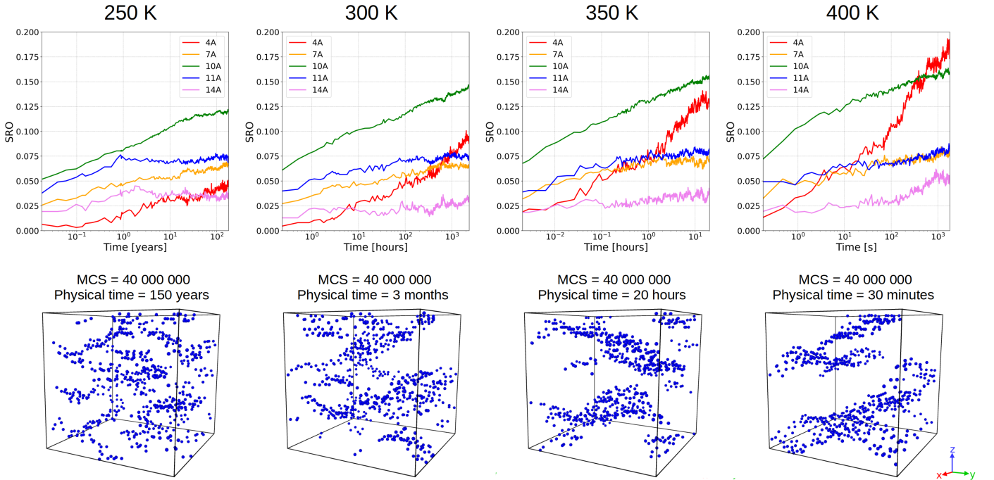
Figure 9: Top: Evolution of short-range order (SRO) parameters in Fe-2C at different temperatures. Bottom: The final carbon distribution obtained in Fe-2C after 40 000 000 Monte Carlo steps (MCS) at different temperatures.
