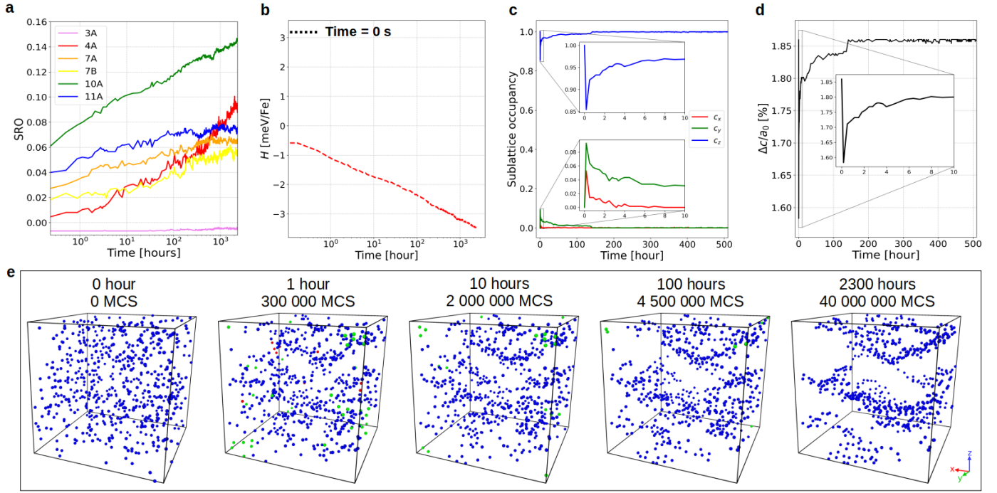
Figure 5: a: Evolution of the short-range order (SRO) parameters. b: Evolution of the system enthalpy. The pair-interaction part of the system enthalpy is the sum over all C-C pair interaction energies. c: Evolution of the sublattice occupancy. d: Evolution of the tetragonality. \Delta c is the variation of the lattice parameter along the tetragonal direction. e: Evolution of the carbon distribution. Red (R), green (G), blue (B) colors refer to site types according to R = x , G = y , B = z . The above simulation results are obtained in Fe-2C (at.%) at 300 K in a 25 \times 25 \times 25 a_0^3 supercell.
