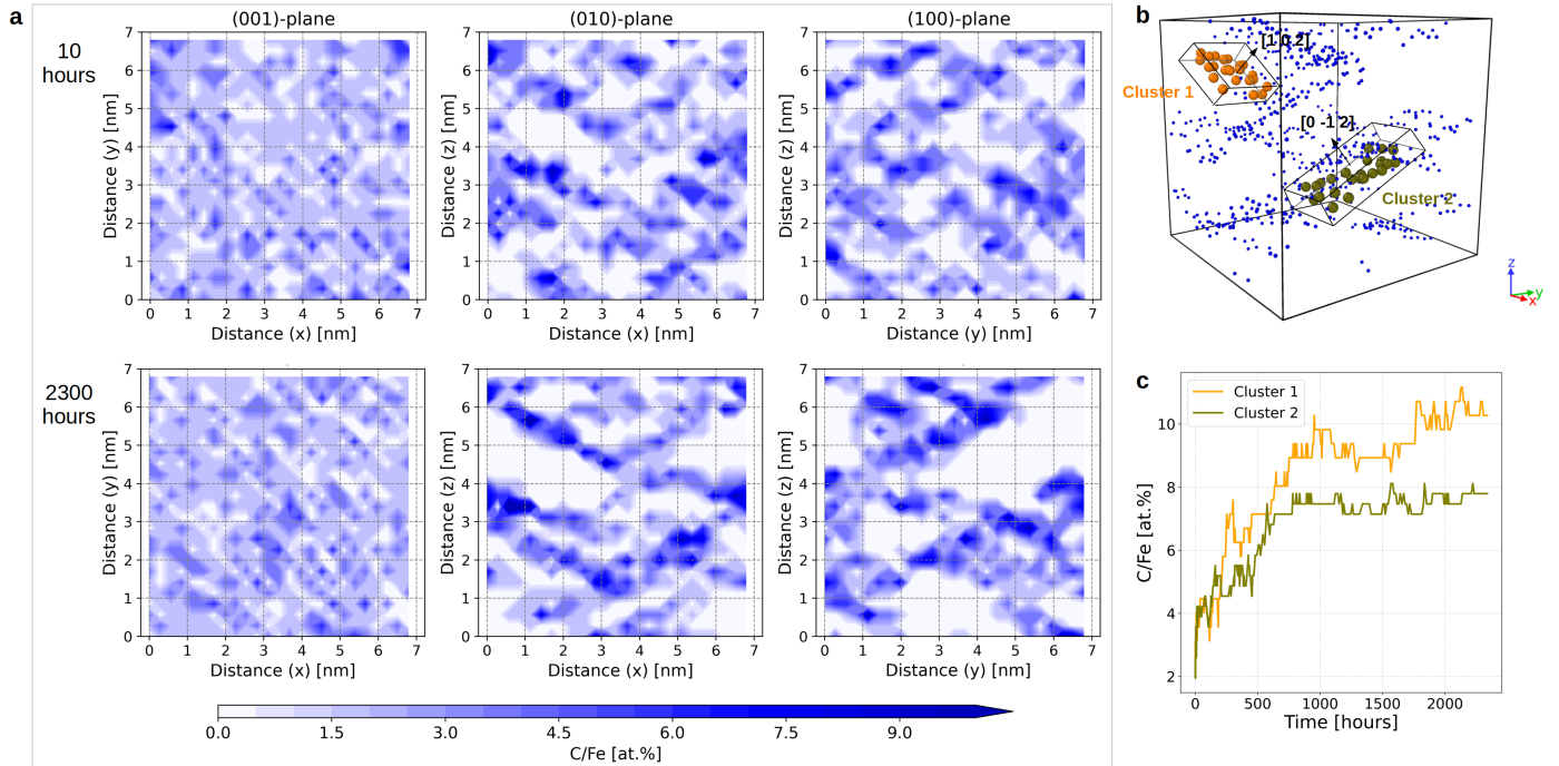
Figure 6: a: Planar distributions of the average carbon concentration in different planes. b: Positions of the two representative clusters. Large spheres (orange and olive) represent carbon atoms within the control volumes of clusters. Small spheres (blue) represent carbon atoms outside these volumes. c: Evolution of the average carbon concentration in the two indicated clusters. These simulation results are obtained in Fe-2C (at.%) at 300 K in a 25 \times 25 \times 25 a_0^3 supercell after 4 \times 10^7 simulation steps.
