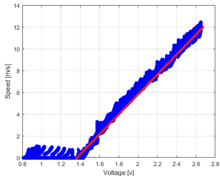
Figure 7. Accelerator vs. motor speed voltage behavior.
