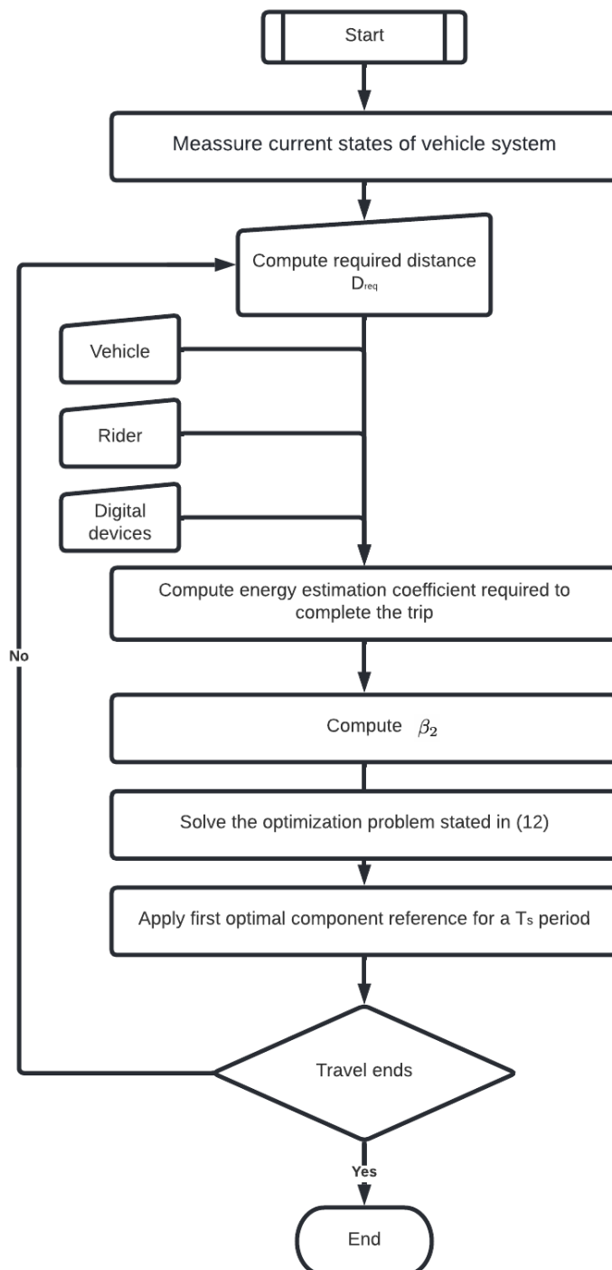
Figure 4. NMPC Algorithm.
