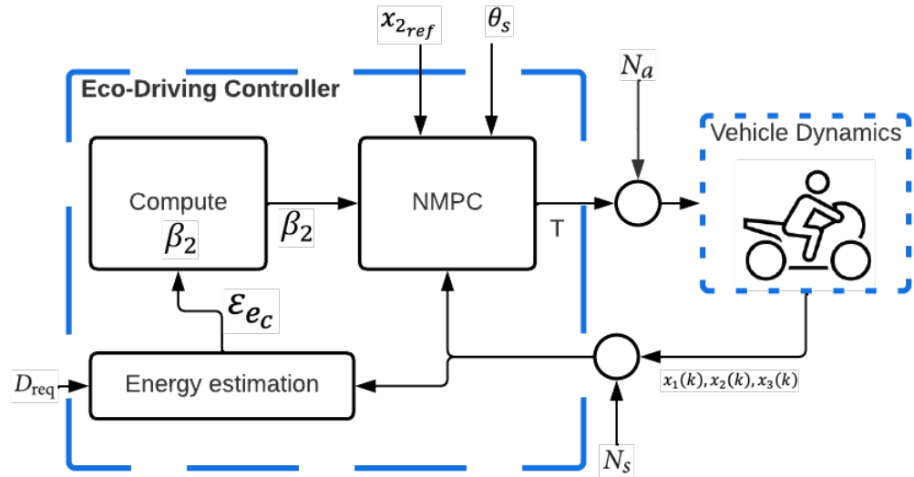
Figure 3. Control Diagram.
