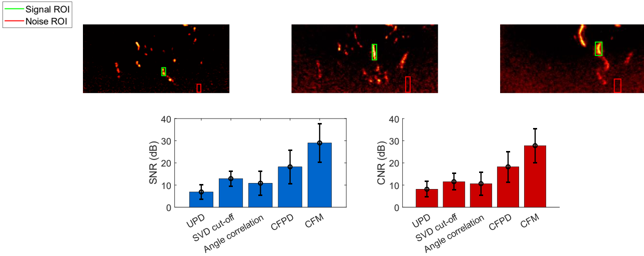
Figure 7 – SNR and CNR measured for the in vivo experiment. The metrics are computed on the three sets of acquisitions presented in Figure 6. The signal and noise ROI are indicated on the corresponding CFM images.
