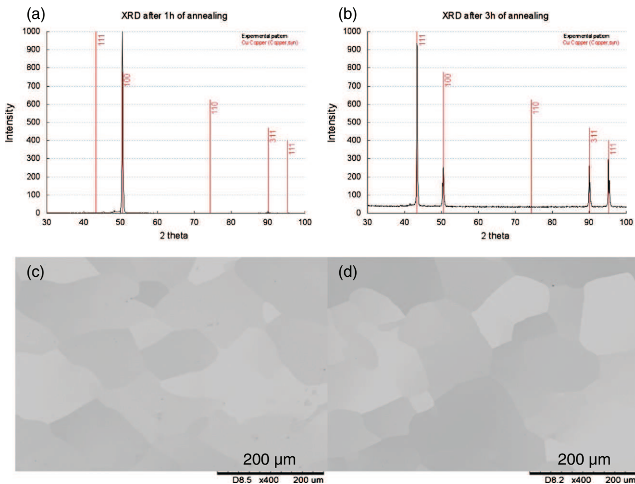
Fig. 1. XRD spectra of copper after (a) 1 h and (b) 3 h of annealing – optical views of copper after (c) 1 h and (d) 3 h of annealing.
