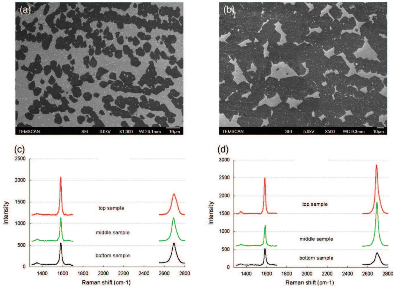
Fig. 2. SEM views of graphene for 120 ppm of methane after (a) 1 h, (b) 3 h of annealing — Raman spectra of graphene after (c) 1 h, (d) 3 h of annealing.
