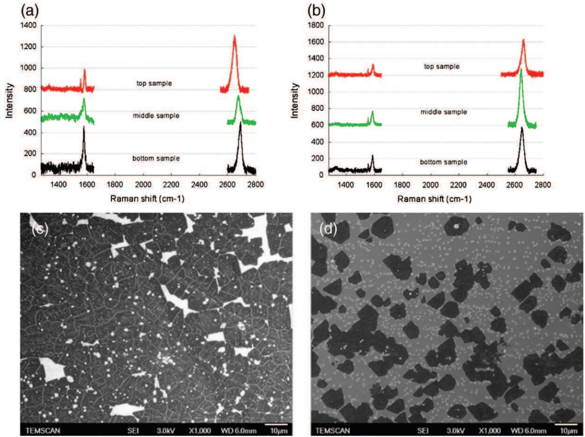
Fig. 3. Raman spectra of graphene formed with (a) 40 ppm, (b) 20 ppm of methane — SEM views of graphene formed with (c) 40 ppm, (d) 20 ppm of methane.
