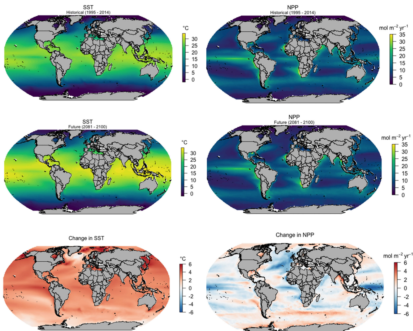
Fig. 1 | Predicted changes in sea surface temperature (SST) and net primary productivity (NPP) for the global ocean. Multi-model mean projections for SST and NPP from 10 CMIP6 Earth system models for the historical period (1995–2014), future (2081–2100) and the change in SST and NPP by 2081–2100 relative to 1995–2014 based on SSP5–8.5. Publicly available datasets were analysed in this
